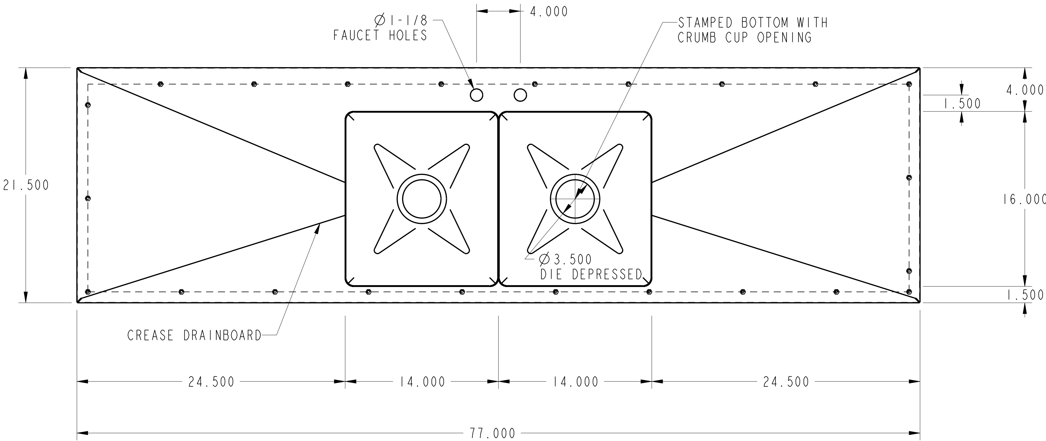
PLAN VIEW
