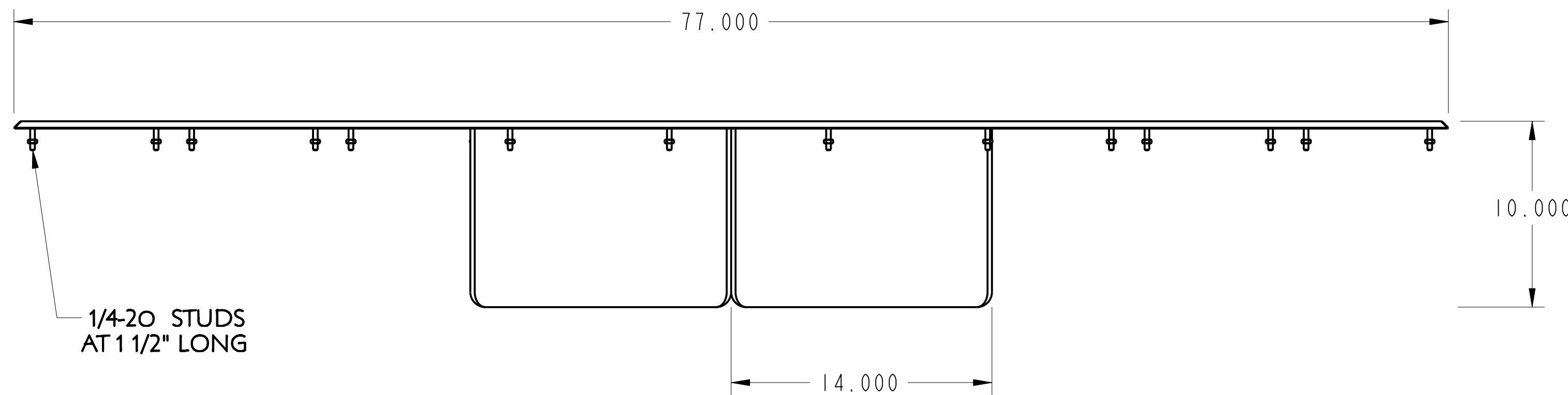
FRONT ELEVATION
